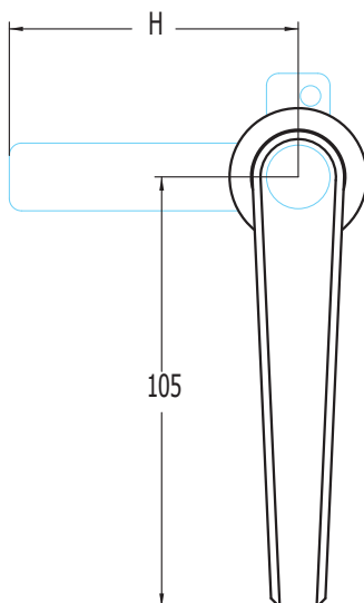
L simple handle with cam for metal cabinets.
