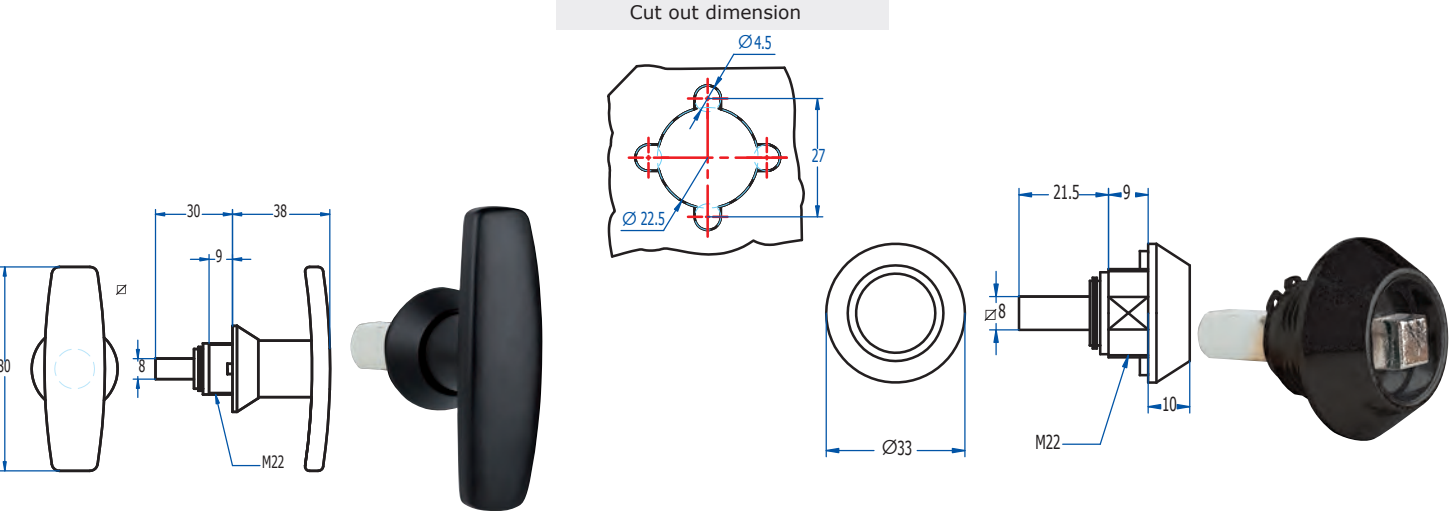
T handle to activate triple point latches.
